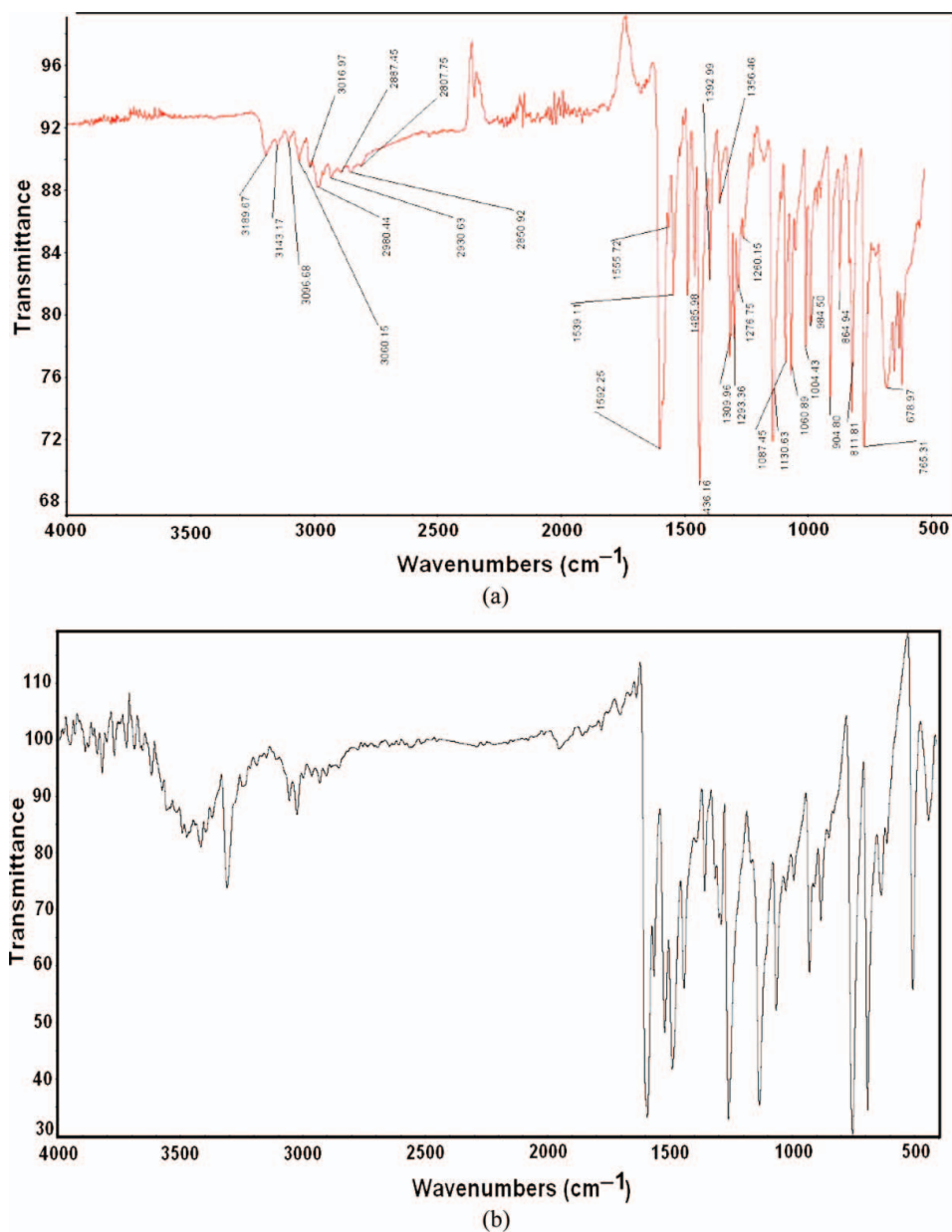
Figure 2. The experimental FTIR spectrum of the (a) BrPyH Schiff base (b) BPH Schiff base.
