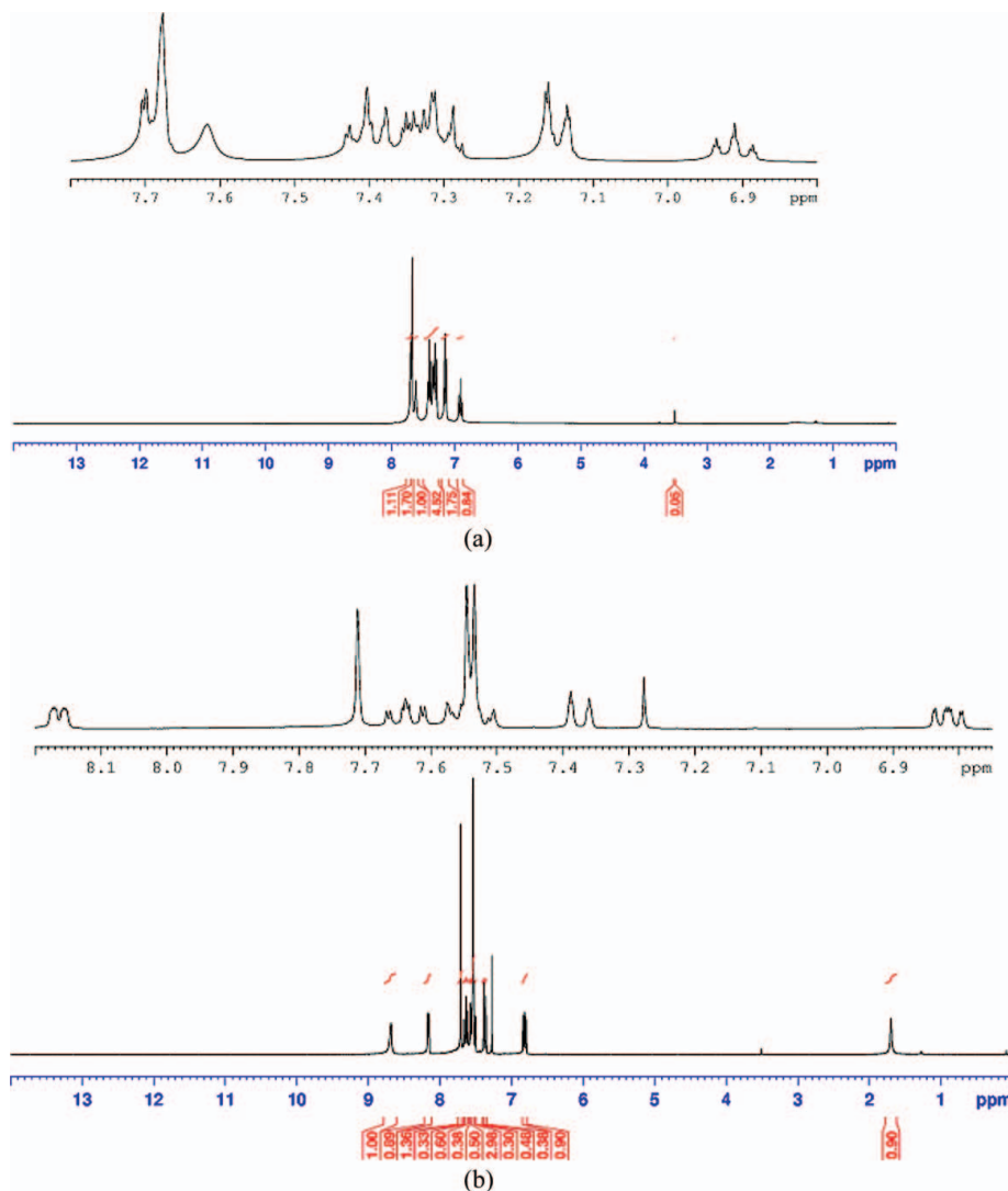
Figure 3. 1 H-NMR spectrum of (a) BPH Schiff base (b) BrPyH Schiff base.
