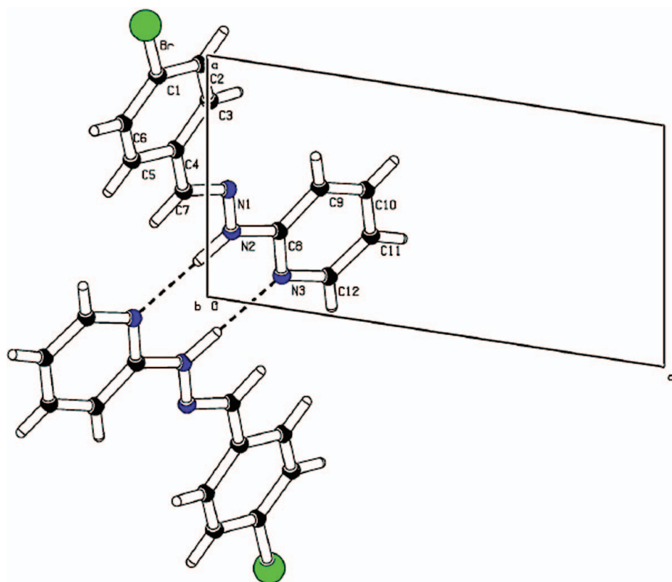
Figure 5. View of the crystal packing of the title compound, along the b -axis. Hydrogen bonds are indicated by dashed lines.
