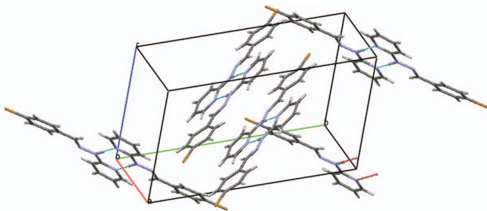
Figure 6. The crystal packing of the compound viewed along a -axis. Intermolecular N—H...N hydrogen bonds are shown as dashed lines.
