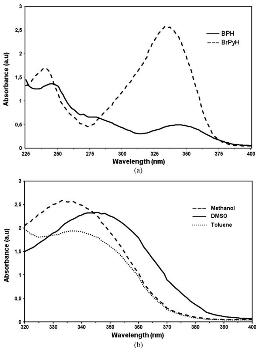
Figure 4. (a) UV–VIS spectra of BPH and BrPyH Schiff bases (in CH_3OH , 10^{-6} M) and (b) UV–VIS spectra of BrPyH Schiff base in various solvents.
