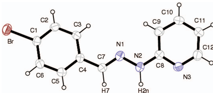
Figure 1. ORTEP drawing of the title compound, represented with displacement ellipsoids, is drawn at 50% probability level and showing the labeling scheme.
